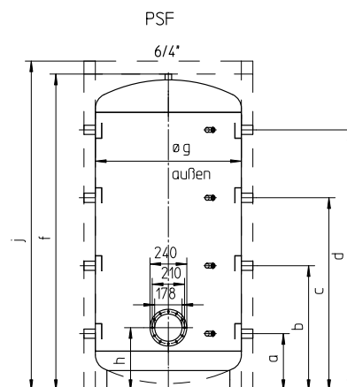
PSF - Pufferspeicher Flansch D 240 500 - 5000l
